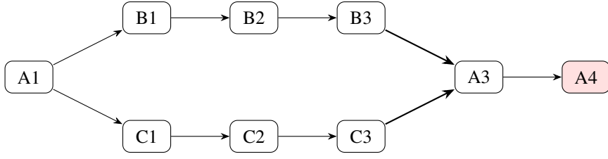
Figure 1: A branching run. A planner (A) starts a researcher (B) and a coder (C). Their outputs merge at A3, which feeds the failing final answer A4. A3 has two parent links, so a simple list or tree cannot represent it.
